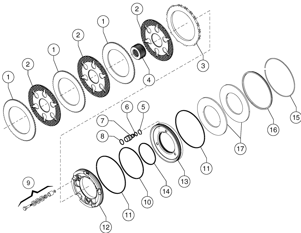
FRONT AXLE - BRAKES
