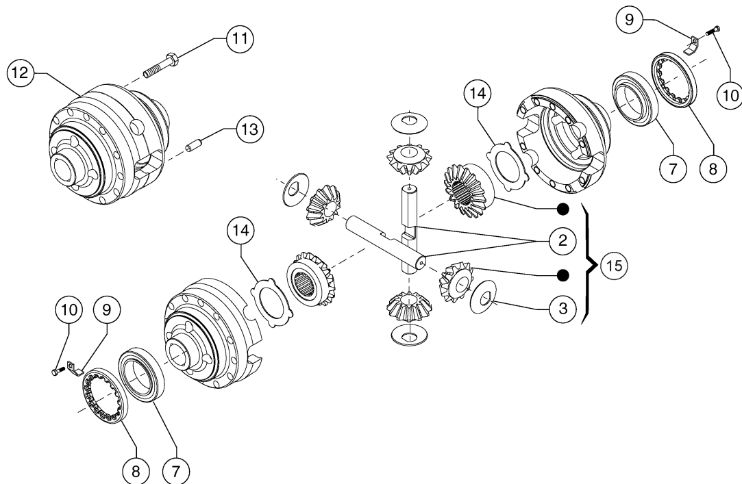
REAR AXLE - DIFFERENTIAL
